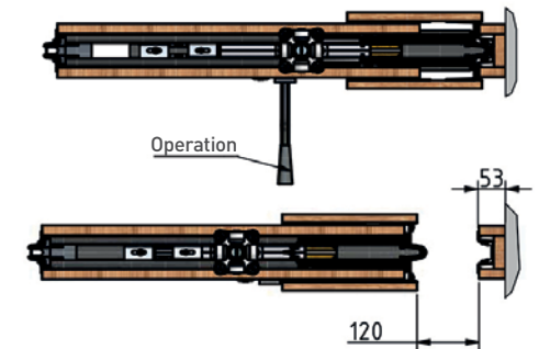
■ Telescopic panel 100 M
