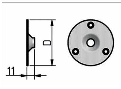
Floor recess plate V2a D=65 mm
