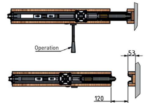
■ Telescopic panel with internal telescopic component
