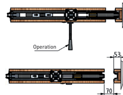
■ Telescopic panel with surface-flush telescopic part
